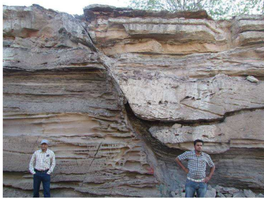
Fig. 16. A N-S trending transverse fault on Bhuj-Kodki road with showing more than 1 m down-throw.
