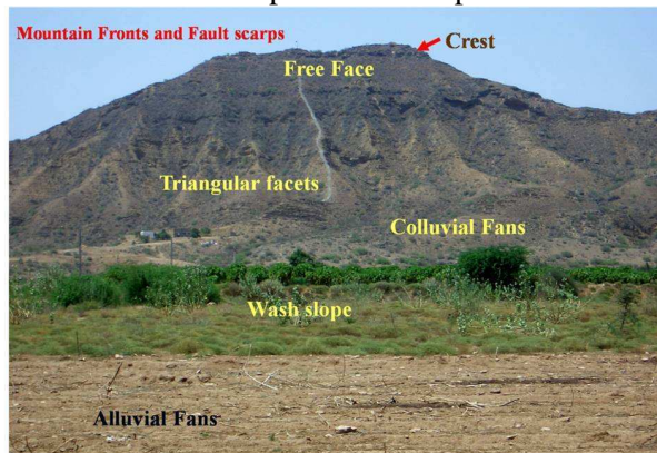
Fig. 23. Khatrod Hill near Kukma village, an ideal site for studying fault scarp morphology.
