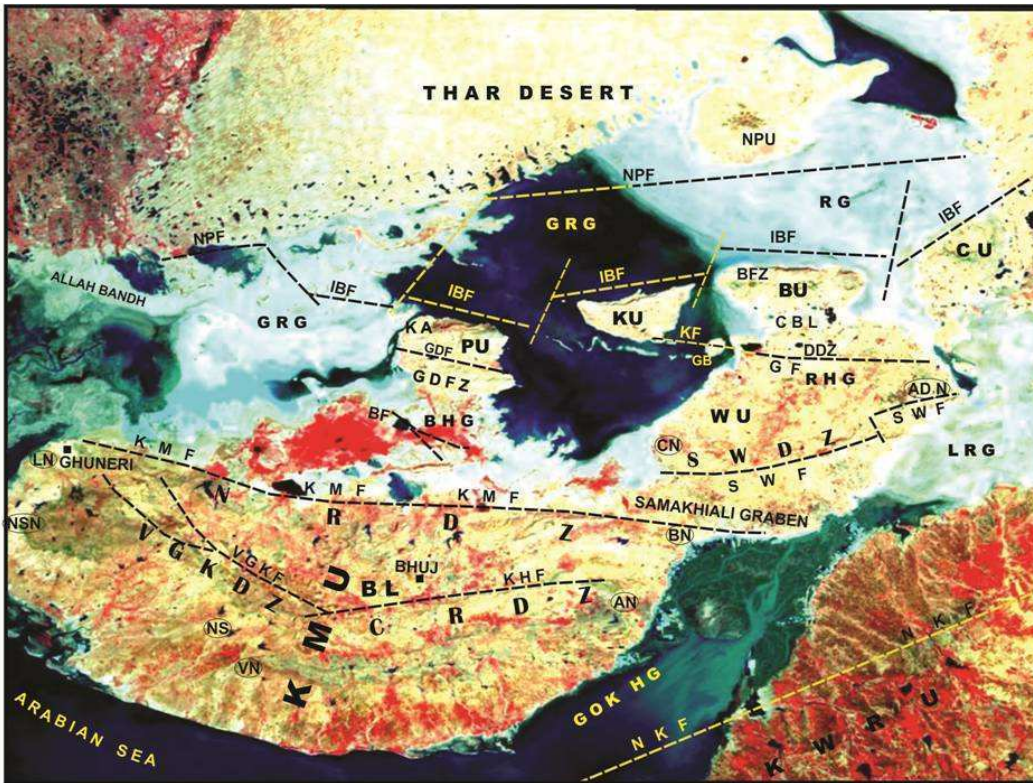
Fig. 6. Morphotectonic map of Kachchh, showing fault-related deformation zones in six uplifts. NPU-Nagar Parkar Uplift , PU-Pachham Uplift, KU- Khadir Uplift, BU-Bela Uplift, CU- Chorar Uplift, WU- Wagad Uplift, KMU- Kachchh Mainland Uplift, NPF- Nagar Parkar Fault, IBF- Island Belt Fault, BHG- Banni Half Graben, BF- Banni Fault, SWF- South Wagad Fault, KMF- Kachchh Mainland Fault, KHF- Katrol Hill Fault, NKF- North Kathiwar Fault, GRG- Great Rann Graben, GOK HG- Gulf of Kutch Half-Graben, GDF- Goradongar Fault, GDFZ- Goradongar Fault Zone, DDZ- Desalpur Deformation Zone, GF-Gedi Fault, BL- Bhuj Low, NRDZ- Northern Range Deformation Zone, RHG- Rapar Half-Graben, SWDZ- South Wagad Deformation Zone, LRG- Little Rann Graben, VGKDZ- Vigodi- Gugriana-Khirasra Deformation Zone, CRDZ- Charwar Range Deformation Zone. KWU- Kathiwar Uplift, KF- Kakindia fault, GB- Gangta Bet. BFZ- Bela Flexure Zone, CBL- Central Balasar Low, LN- Lakhpat Nose, NSN- Narayan Sarovar Nose, AN- Anjar Nose, BN- Bhachau Nose, CN- Chobari Nose, ADN- Adesar Nose.
