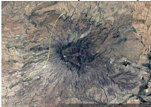
Fig. 33. A Google Earth view of the Dhinodhar Plug with radial drainage pattern.
