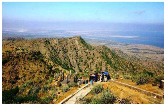
Fig. 29. A panoramic view of the N-facing scarp of Kaladungar Hill range and the Great Rann of Kachchh beyond.
