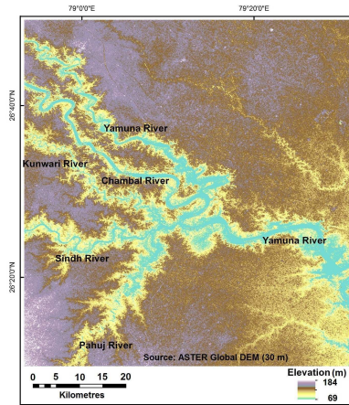
Fig. 7. ASTER DEM (30 m) of the ravines along the Chambal River and its major tributaries near the Chambal-Yamuna confluence.
